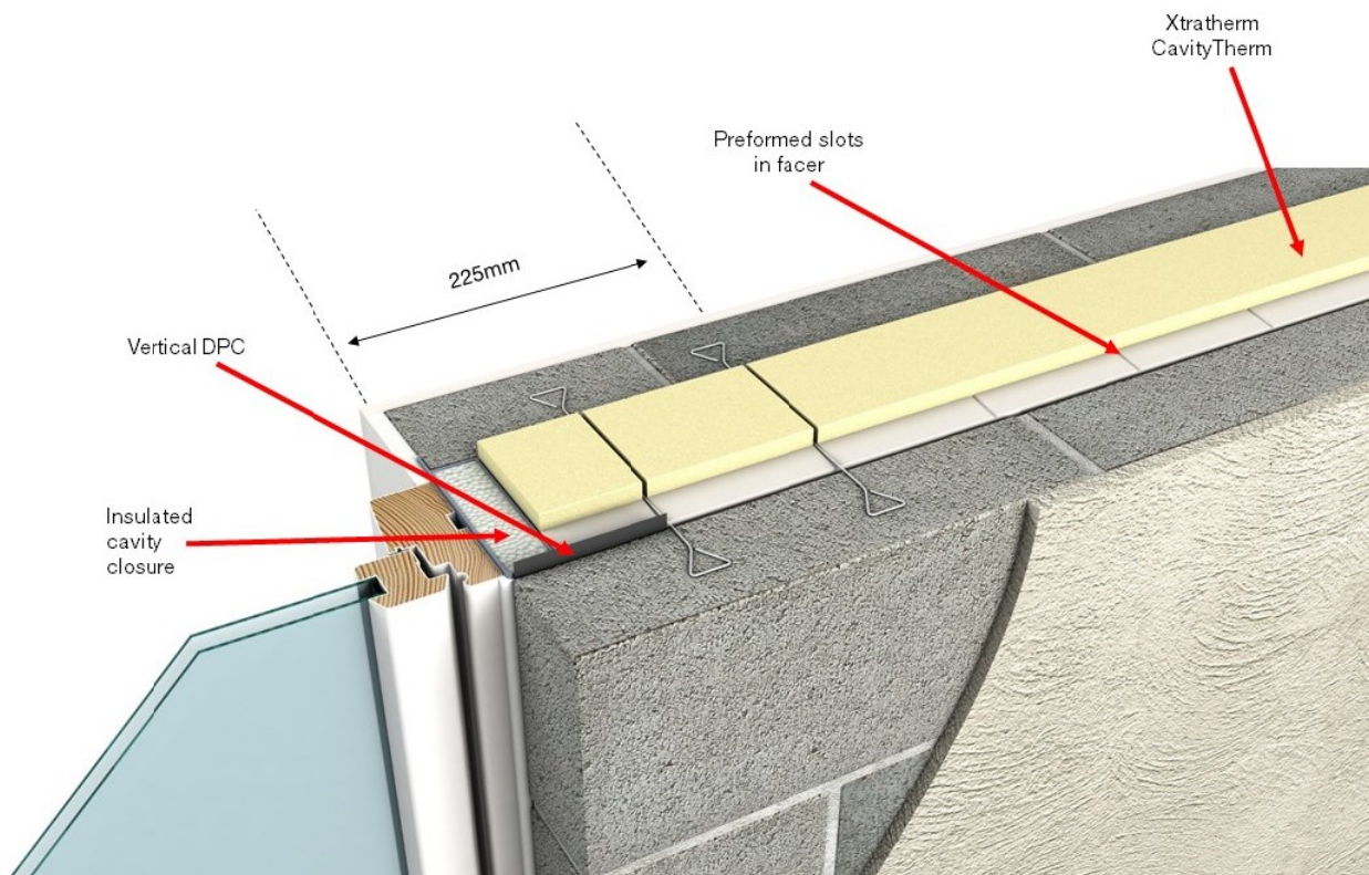
Figure 7 – Installation of Additional Wall Ties Windows/Door Openings.
