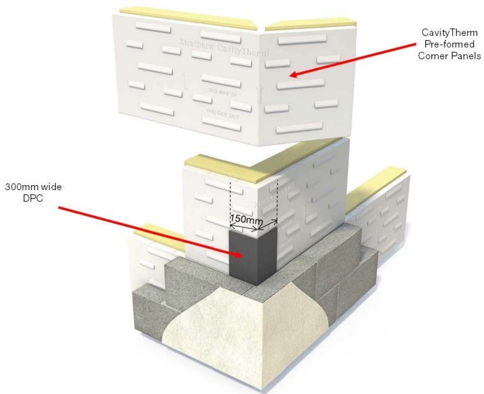
Figure 4 – Installation Detail at Corners Including Xtratherm Pre-formed Corner Panels.
