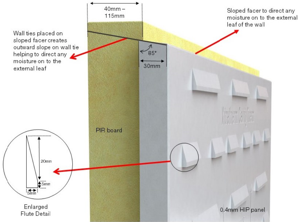
Figure 2 – Xtratherm CavityTherm Panel – Profiled Edge and Drainage Detail
