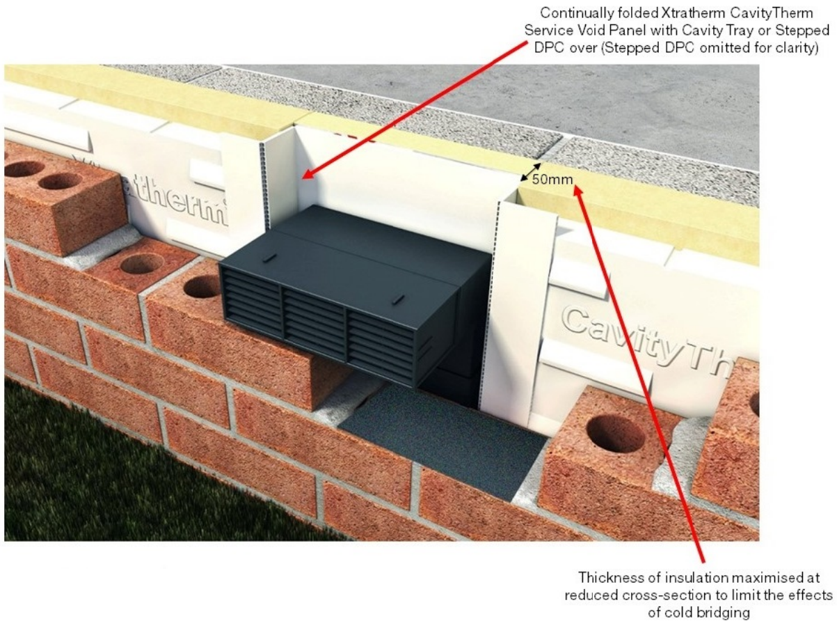
Figure 10 – Xtratherm Subfloor Services/Ventilation Panel. (Cavity tray/flashing not shown for clarity) .
