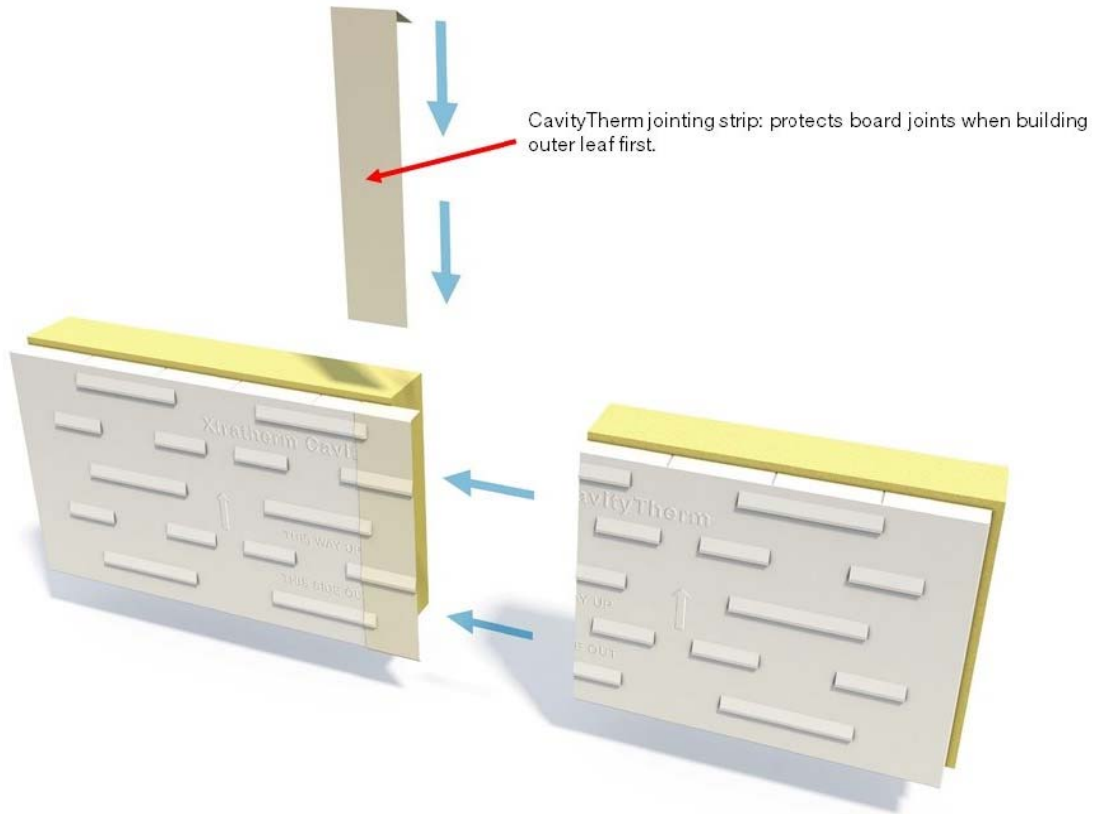
Figure 8 – Xtratherm CavityTherm Jointing Strip.
