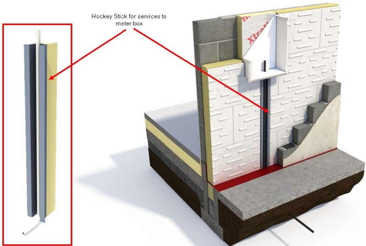
Figure 5 – Xtratherm CavityTherm Hockey Stick & Meter Box Board Installation Detail.
