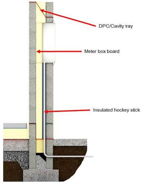
Figure 6 - Xtratherm CavityTherm Meter Box Board Cross-section Including Typical DPC/Cavity Tray Installation Detail.
