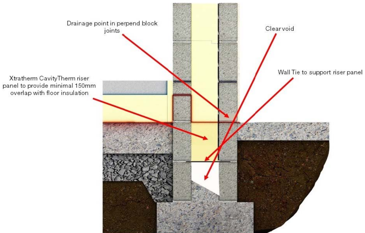
Figure 3 - Typical Installation Detail Including XtraTherm Riser Panel.
