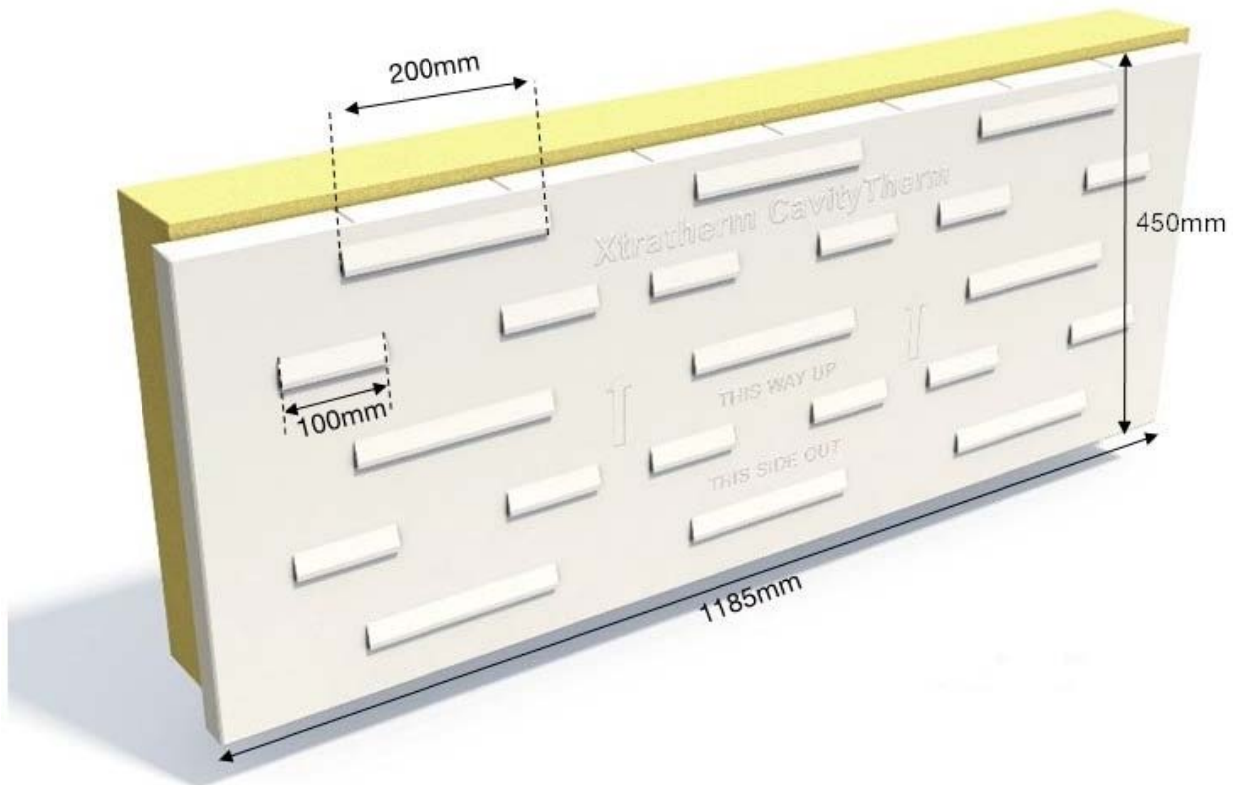
Figure 1 – Xtratherm CavityTherm Panel – Front elevation.
