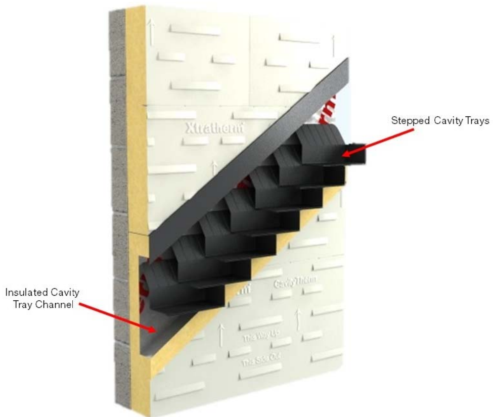
Figure 9 – Xtratherm Insulated Cavity Tray Channel.
